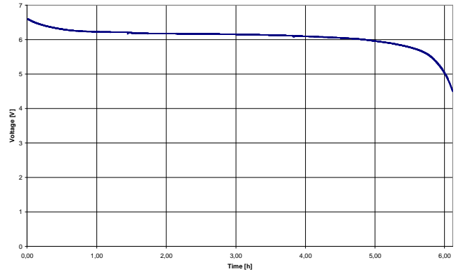
Run time for SL20XPLED 2,4Ah rechargeable battery
